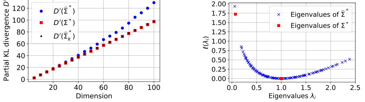
(a) Evolution of the partial KL divergence as the dimension increases, with the optimal covariance matrix \Sigma^* (red squares), the sample covariance \hat{\Sigma}^* (blue circles), and the projected covariance \hat{\Sigma}_k^* (black dots).
