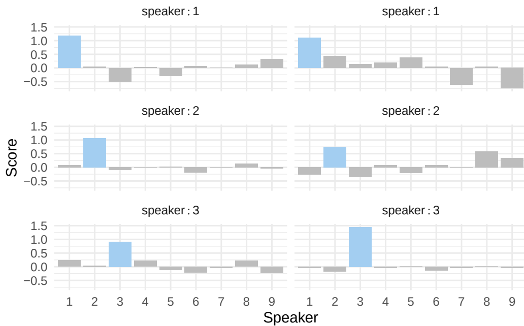
Figure 11: Prediction in a sequence-to-sequence approach 6 samples with 3 speakers and 2 utterance each. The speaker to predict is depicted in blue. For each of the 6 utterance, the model correctly identifies the speaker.
