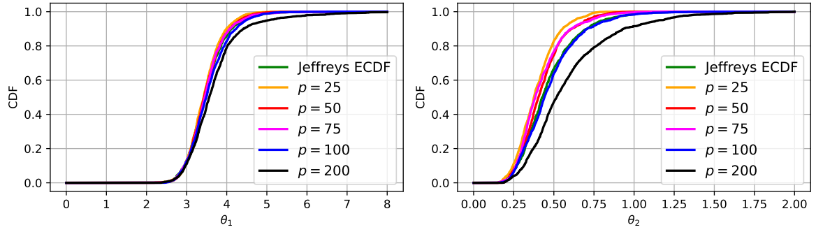
Figure 17: Empirical cumulative distribution functions for the unconstrained fitted posterior and the Jeffreys posterior using 5000 samples. The band is obtained by computing the ECDFs over 100 different seeds and monitoring the maximum and minimum ECDF values for each \theta .
