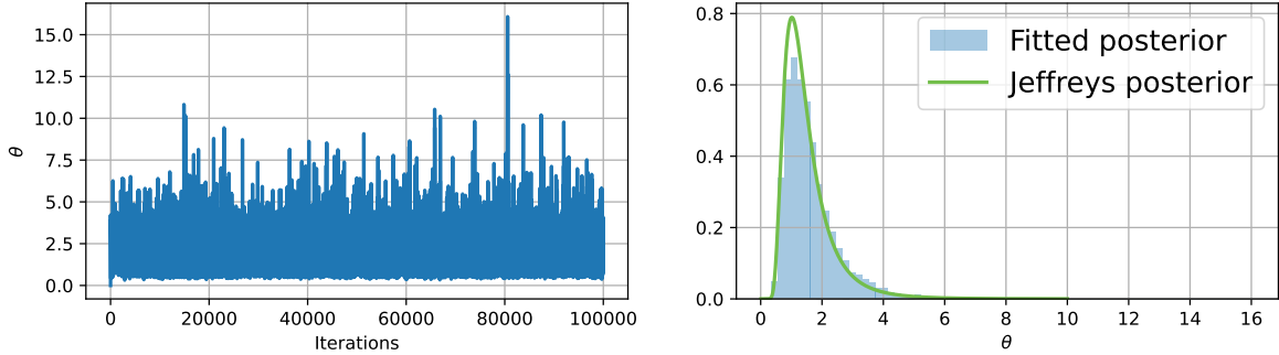
Figure 10: Left: Markov chain during the Metropolis-Hastings iterations. Right: Histogram of the fitted posterior obtained from 5 \cdot 10^4 samples and the density function of the Jeffreys posterior.
