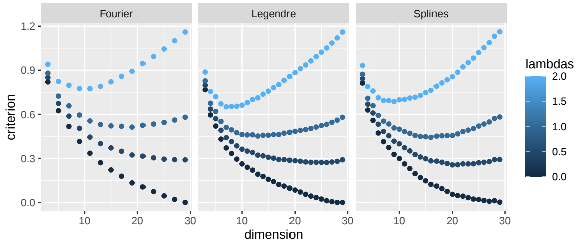
Figure 5: Illustrative example. For a given simulated dataset, we show the behavior of the criteria as a function of dimension L, for several lambdas, for Fourier (left), Legendre (middle) and Splines (right) basis.
