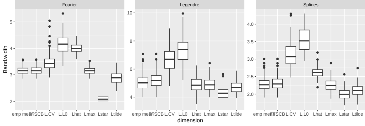
Figure 7: Illustrative example. We display within boxplots the confidence band's width over 100 repetitions for the dimension selected by the several criterion introduced in this paper, for Fourier (left), Legendre (middle) and Splines (right) basis.
