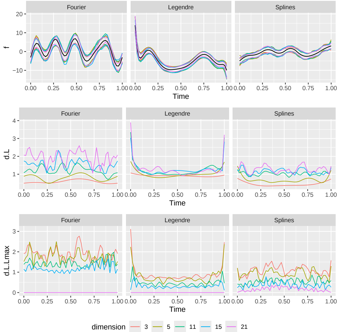
Figure 3: Illustrative example. For a given dataset, we plot several confidence bands (top row), functions dL (middle row) and dLL_{max} (bottom row). Bands and functions are estimated with Fourier (left column), Legendre (middle column) and Spline (right column) basis and several dimensions L (3, 5, 11, 15, 21).
